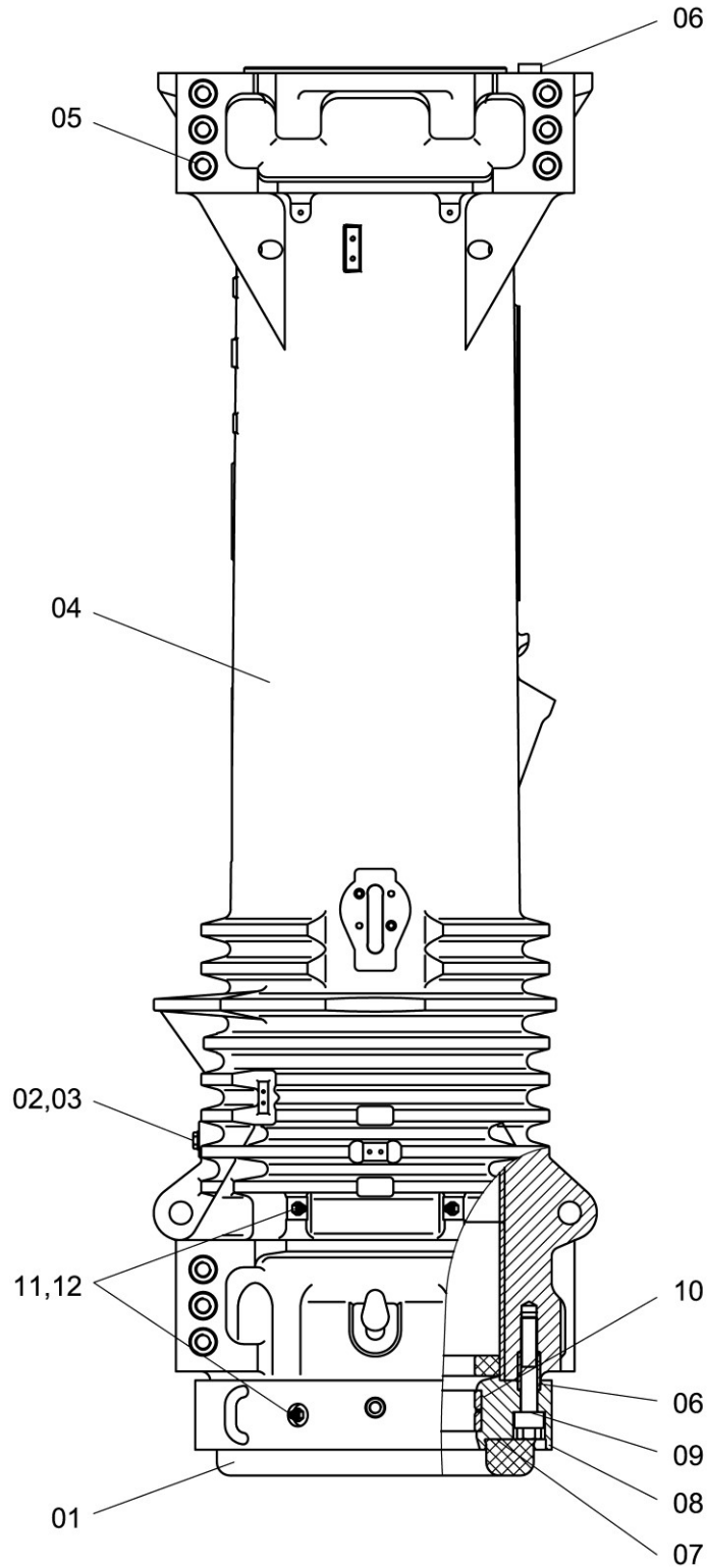
Hera D62-22 Lower cylinder
