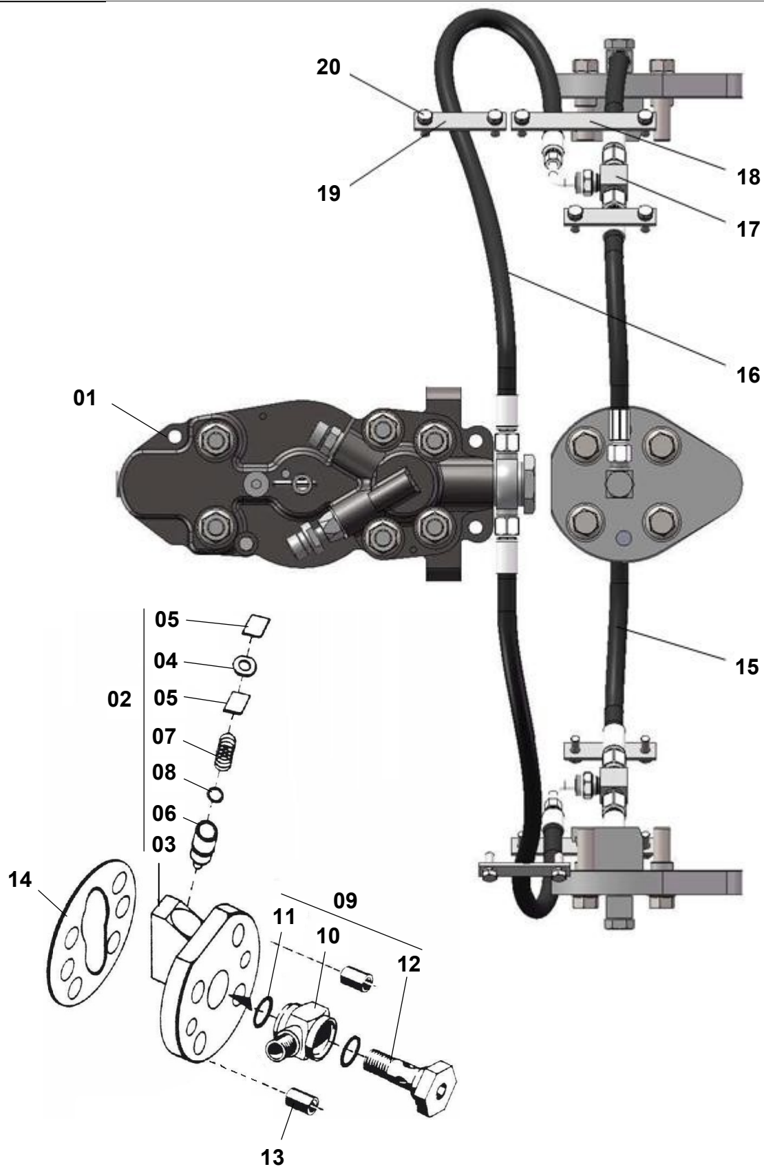
Hera D80/D100-13 Fuel injection device
