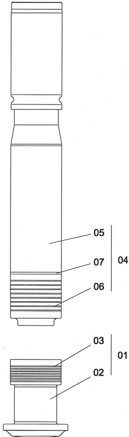
Hera D80/D100-13 Impact block complete
